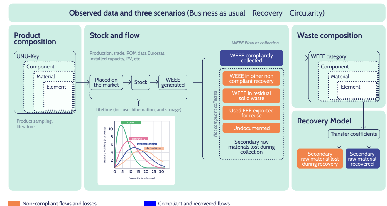
Figure 1 - Main steps of the applied methodology (adapted from the FutuRaM project, see Iattoni et al., 2025 and Yamamoto et al., 2025).
