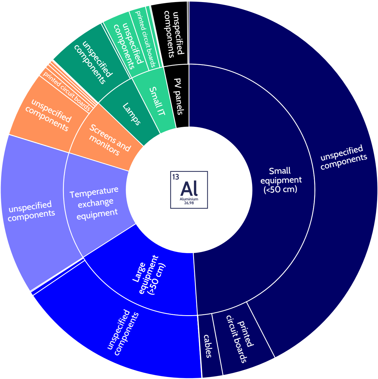
Figure 12 - Main aluminium applications across WEEE categories and components (reference year: 2022).
