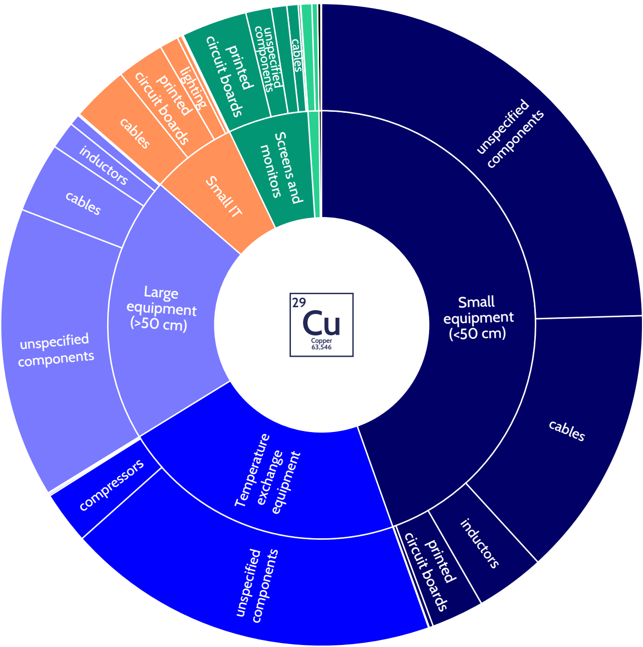
Figure 14 - Main copper applications across WEEE categories and components (reference year: 2022).
