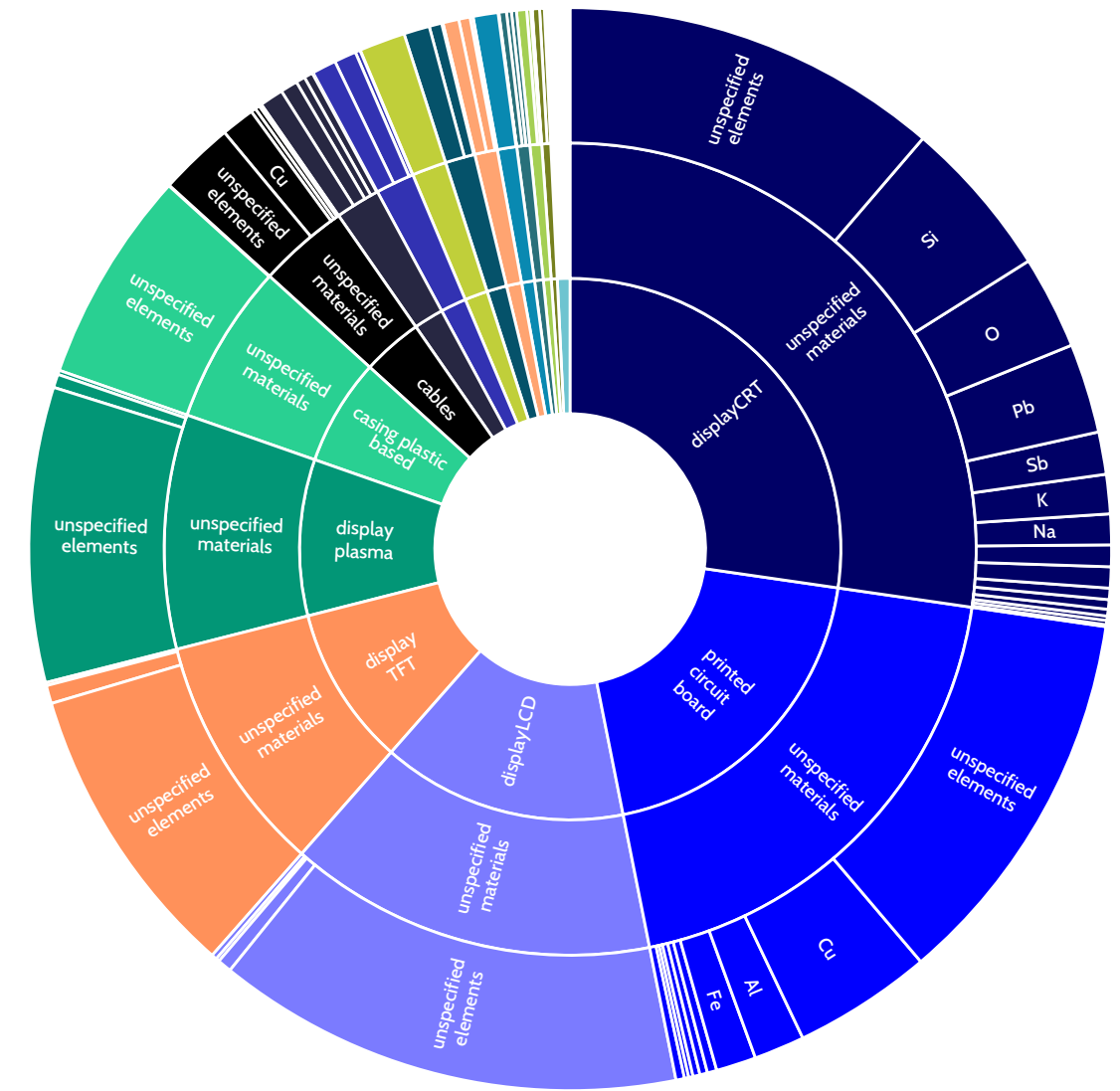
Figure 4 - Hierarchical distribution of composition data (p–c–m–e) aggregated for the WEEE category Screens and monitors. All components, materials, and elements are shown except the item «unspecified components» and the related materials/elements embedded, which was removed to improve visibility. This chart therefore covers approximately 37% of the total composition. 10
